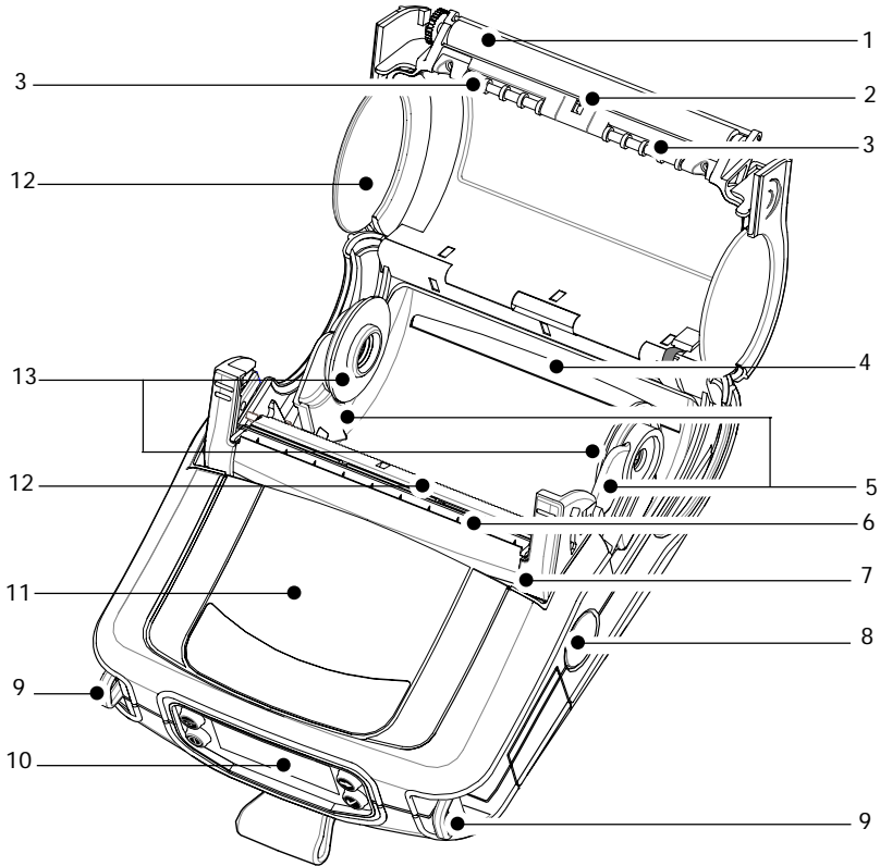
Figure 1C: QL 420 Overview
